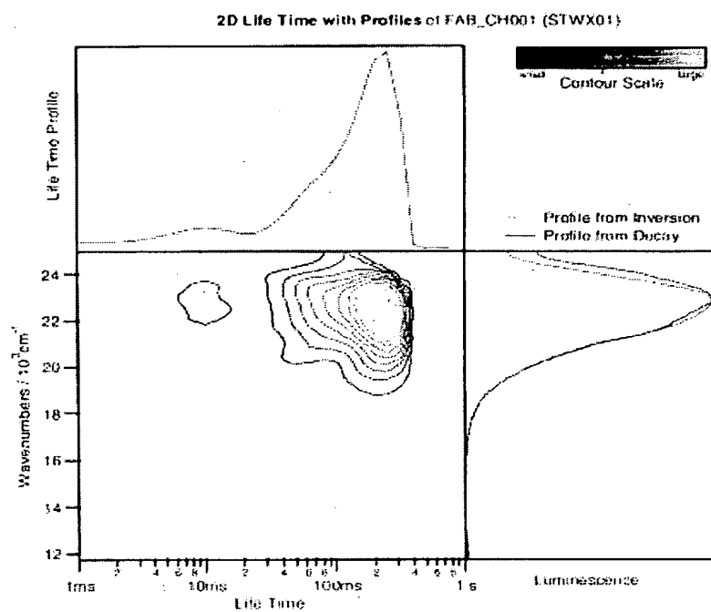
FIGURE 5 FAB in Cyclohexane at 80K
